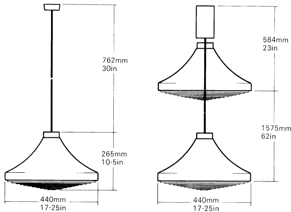
WZA Rise and fall, also cable suspension
