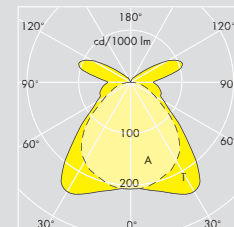
Cat. No. DLUX CZ 158 Lamp: 1 x 58W T8 DLOR: 0.64 LOR: 0.81 SHR max: 2.03 LMG: E
